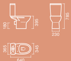
SANITA compacta D/P
