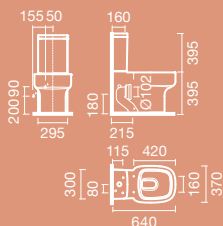
SANITA compacta BTW
