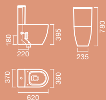
SANITA compacta BTW
