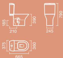
SANITA compacta
