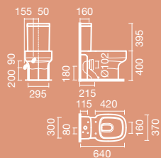
SANITA compacta
