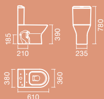
SANITA short BTW
