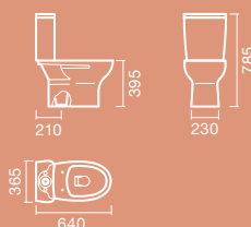
SANITA compacta D/C
