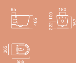
SANITA suspensa
