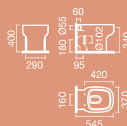
SANITA simples BTW
