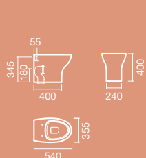
SANITA simples BTW
