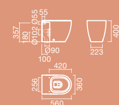
SANITA simples BTW
