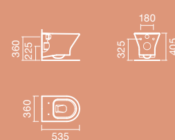
SANITA suspensa
