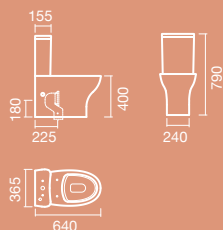
SANITA compacta BTW
