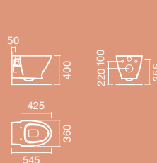
SANITA suspensa
